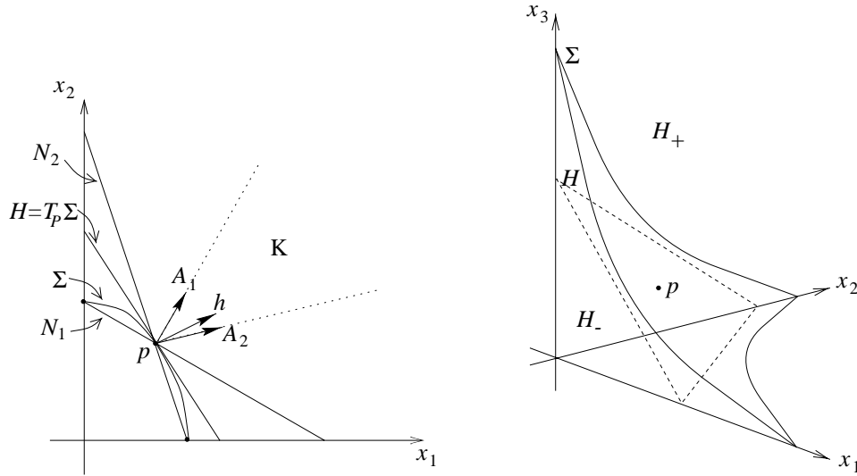
FIGURE 4. In the figure on the left, \Sigma and T_p\Sigma lie between the nullclines, and so h lies in the convex hull K of the A_i^T . The figure on the right shows \Sigma and H = T_p\Sigma for a three-dimensional example in which \Sigma \setminus p lies in H_+ .
